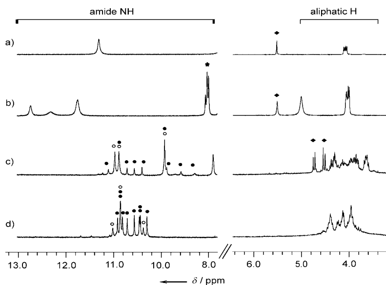
Figure 2. Excerpts of ^1\text{H} NMR spectra at 298 K of: a) 2 (5 mM) in \text{CDCl}_3 ; b) 1 (5 mM) in [\text{D}_3]\text{pyridine} ; c) 1 (5 mM) in \text{CDCl}_3 ; d) 1 (5 mM) in \text{CD}_3\text{CN} . Signals of the triplex in parallel and antiparallel configurations are marked with open ( \circ ) and filled circles ( \bullet ), respectively. Methylene protons of benzyl ester groups are indicated by diamonds ( \blacklozenge ). The water peak in pyridine appears at around \delta = 5.1 ppm. A few aromatic signals are marked with a star.
