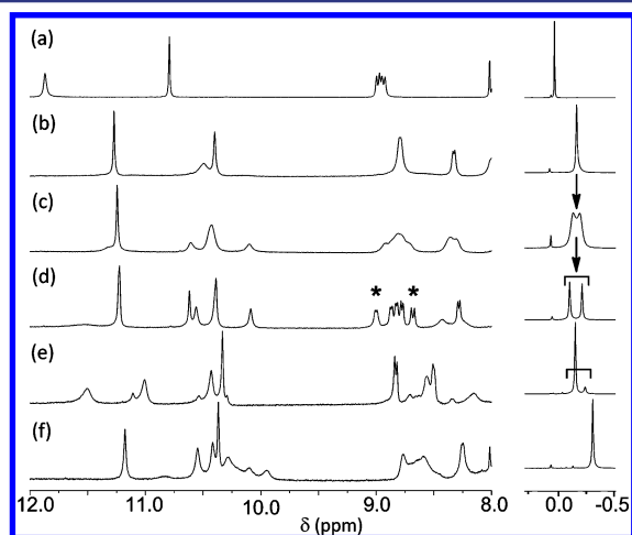
Figure 3. Parts of the 300 MHz ^1H NMR spectra of 1 and the 400 MHz ^1H NMR spectra of 2 and 3 showing aromatic amide resonances (10–12 ppm), some aliphatic amide and aromatic proton resonances (8–9 ppm), and TMS resonances (–0.5 to 0 ppm): (a) 1 at 25 °C in CDCl_3 ; (b–d) 2 at 45, 25, and 5 °C in CDCl_3 ; (e) 2 at 5 °C in CD_3CN ; (f) 3 at 25 °C in CDCl_3 . The stars indicate two leucine NH protons having very different ^3J_{NH-C^\alpha H} coupling constants.
